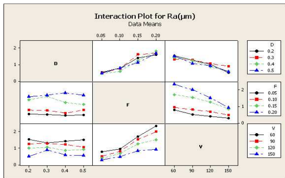
Figure 3 Interaction Plot for surface roughness (Ra)
