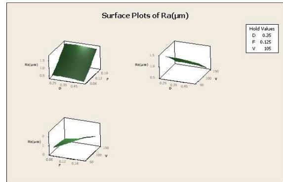
Figure 5 Surface Plots for surface roughness (Ra)
