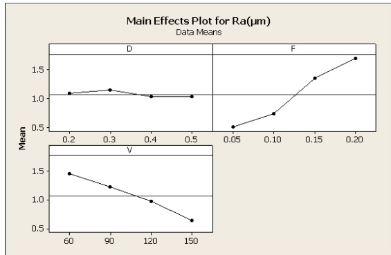
Figure 2 Main Effects Plots for surface roughness
