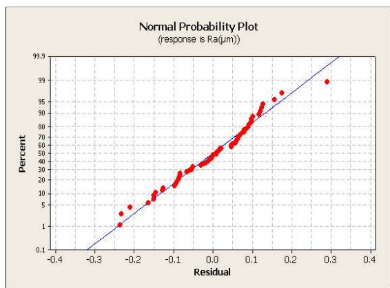
Figure 6 Normal Probability of the residuals for surface roughness (Ra)
