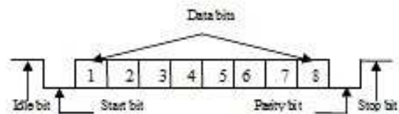
Figure 1. UART Frame Format
