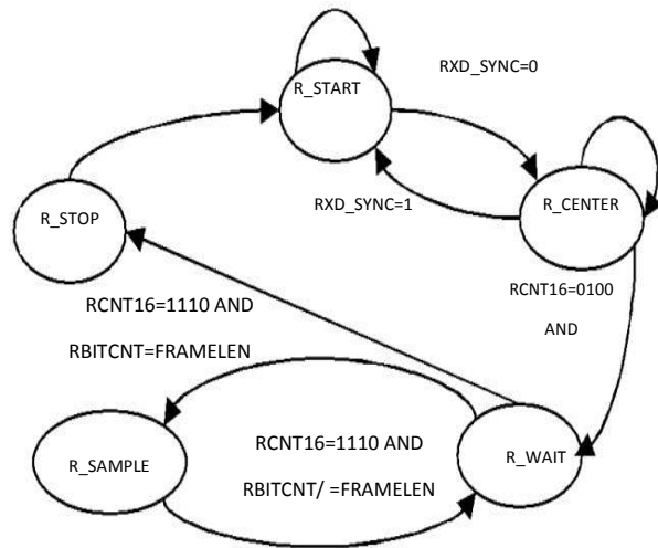
Figure 3. UART Receiver State Machine
