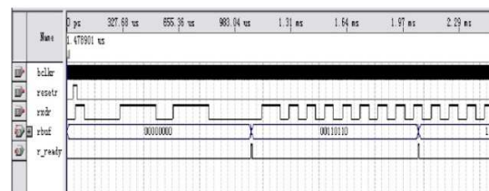
Figure 6 Receiver Simulation Diagram
