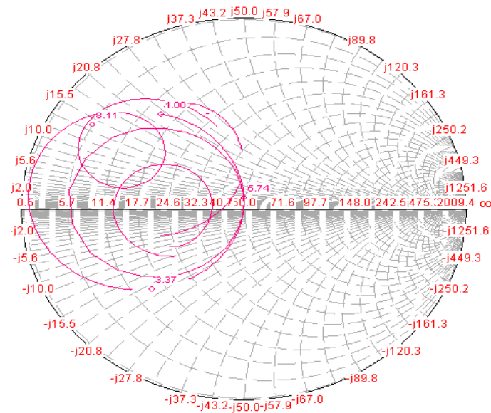
Figure 4. Input impedance loci using smith chart for iteration I
