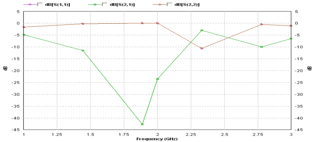
Figure 3. Return loss vs. frequency of iteration I for proposed antenna
