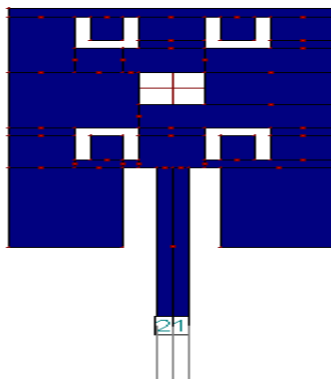
Figure 2. Geometry of iteration 1 with t=1.524 , Permittivity=4.4 and grid size=.025 , l=20 , w=20 , feed length=20mm, feed width=2mm..
