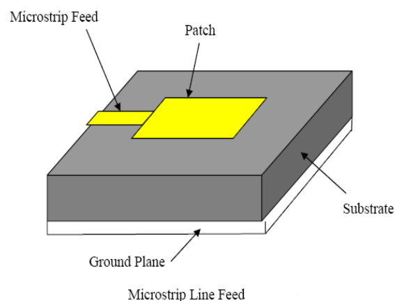
Figure 1: Microstrip line feed
