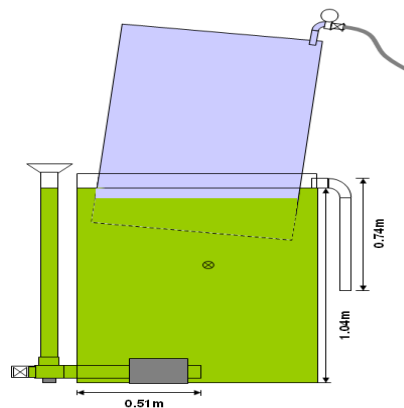
Fig 2. Final State of Plant when Methane is produced in Gas holder tank
