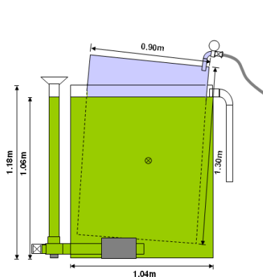
Fig 1. Initial State of Plant
