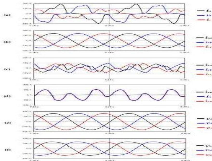
Figure 4. Typical waveforms of an installation with a UPQC: (a) Load currents; (b) Source currents; (c) Compensation currents; (d) Neutral wire currents; (e) Load voltages; (f) Source voltages
