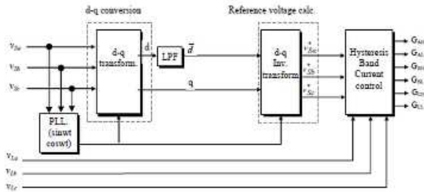
Fig. 2 Block diagram of series APF control
