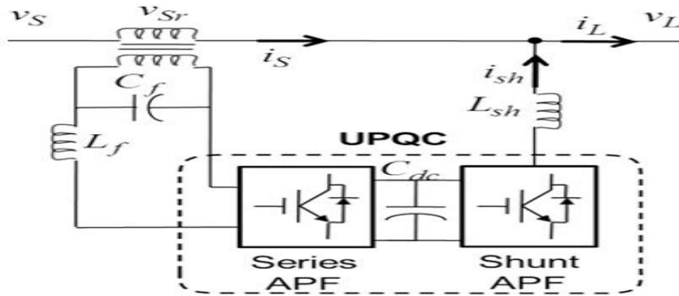
Fig.1 Unified Power Quality Conditioner configuration
