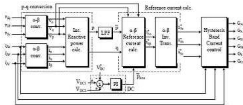
Fig. 3 Block diagram of shunt APF control
