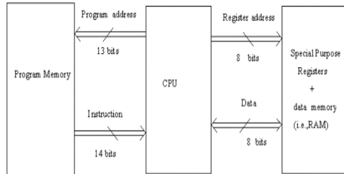
Fig. Architecture of PIC microcontroller
