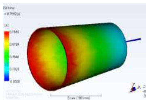
Fig .6B)Fill Time Analysis result
