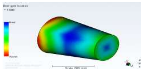
Fig. 6A ) best gate location
