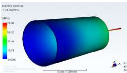
Fig . 6E )Injection Pressure result fig .
