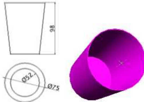
Fig5.1 a). CAD Model Of Plastic CUP
