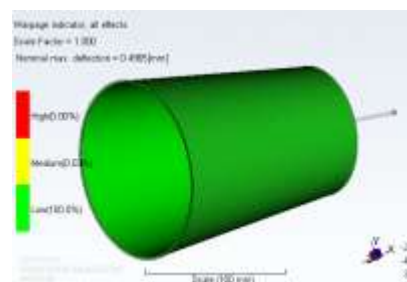
Fig.6M ) wrap analysis result
