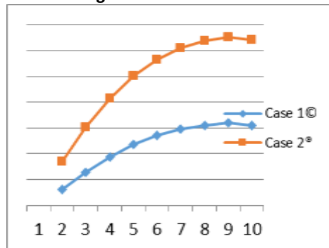
Fig:3.13:- Shows Drift Value along X Direction for load combination 0.9DL+1.5(+X).
