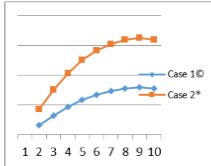
Fig:3.11:- Shows Drift Value along X Direction for load combination 1.5(DL+(X)).
