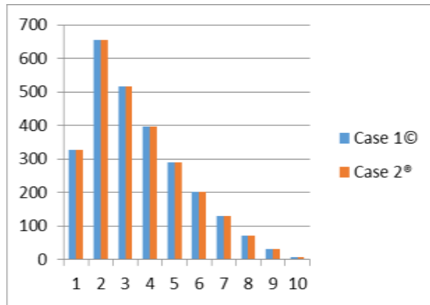
Fig.3.3: - Story shear along X direction
