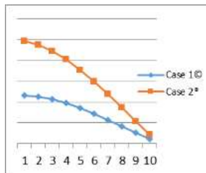
Fig:3.5: - Shows Corner Edge Displacement Value along X Direction for load combination 1.5(DL+(X)).
