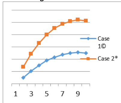
Fig:3.12:- Shows Drift Value along X Direction for load combination 1.2(DL+LL+ (+X)).
